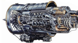
TFE 731 Engine
